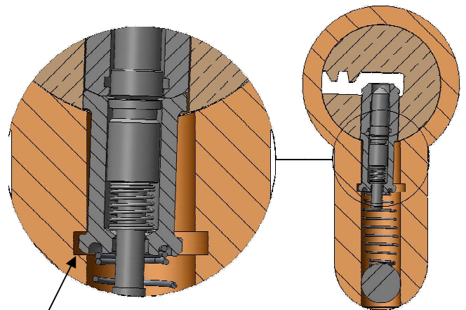
Special groove in the body chamber
