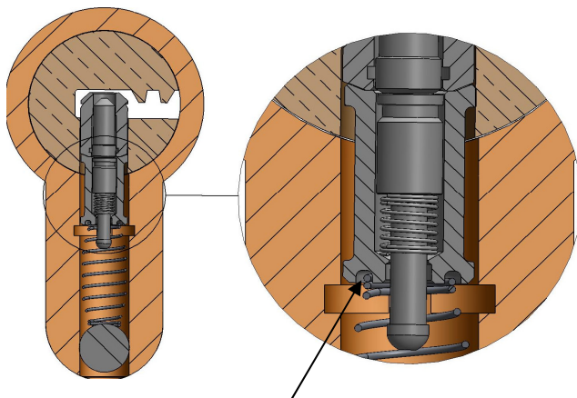
Special groove in the pin
